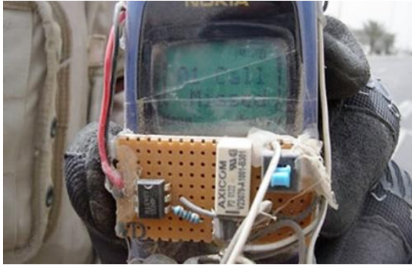
IED; Improvised Explosive Device
